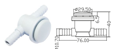
Twin Hole Air Jet
