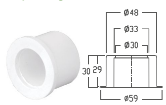
Pipe Plug
