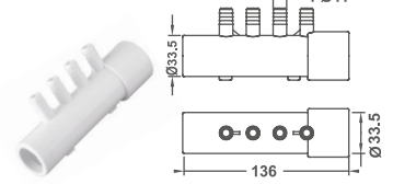
Port Air Manifold
