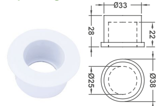
Pipe Plug
