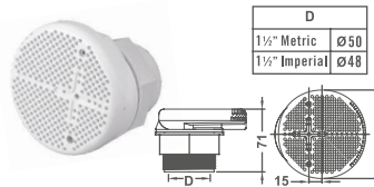
φ2 Section Drain Lock Nut
