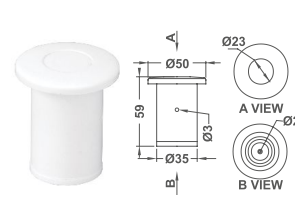
Air Button
