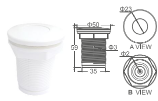
Air Button
