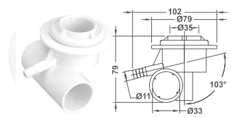
φ10mm Barb Air & φ25mm Water
