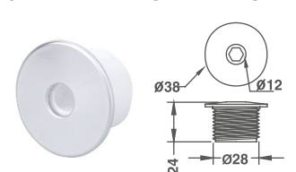
φ1-1/2" Face (Standard) Jet
