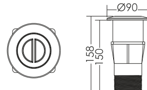
Vacuum Fitting (Concrete Pool)
